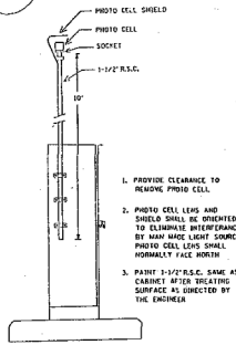
PHOTO CELL DETAIL
