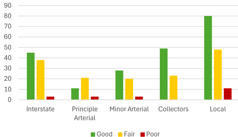
Figure 30: Structure Condition by Functional Class
