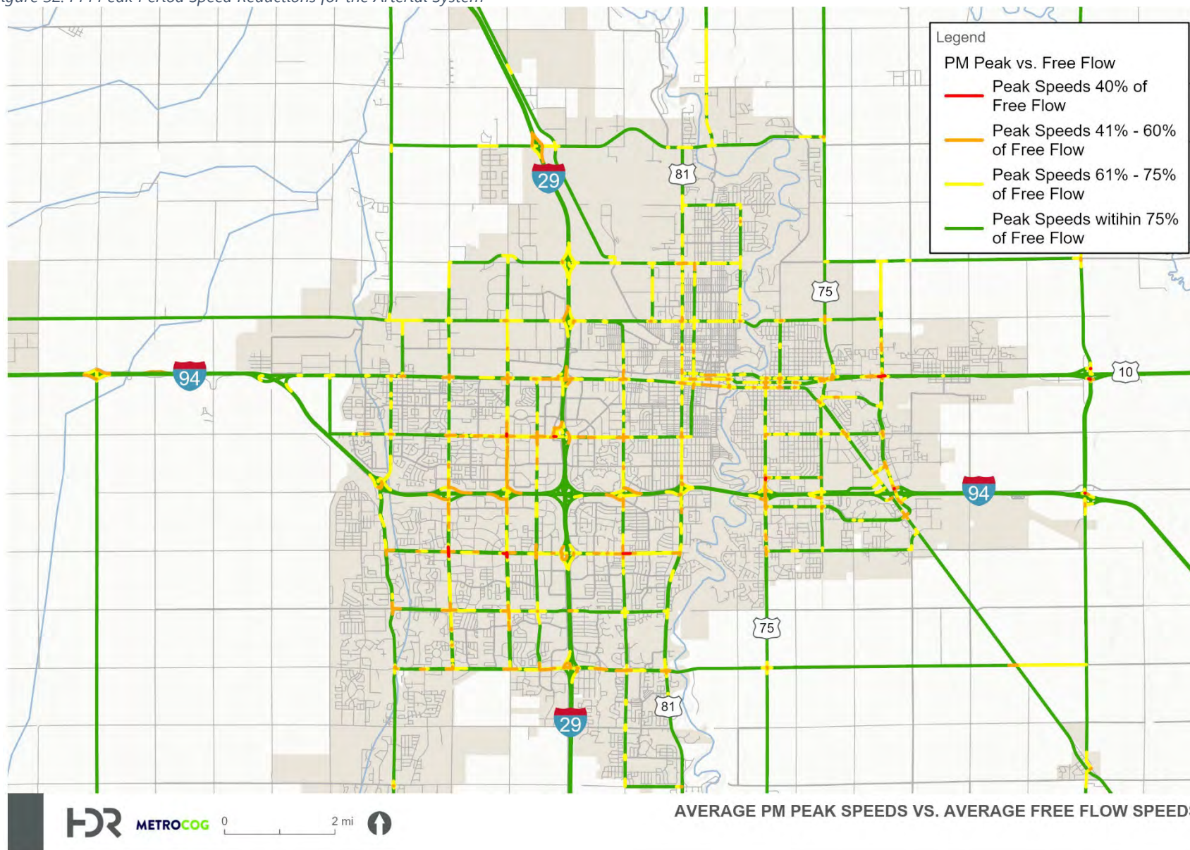
Figure 32: PM Peak Period Speed Reductions for the Arterial System
