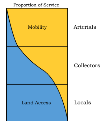
Figure 10: Mobility and Accessibility Characteristics of Functionally Classified Roads
