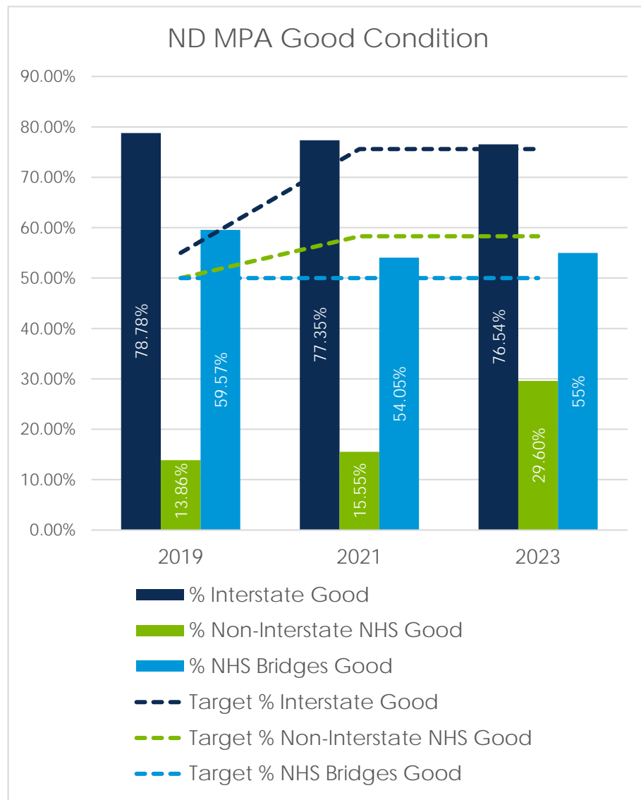
Figure 8. ND MPA PM 2 Performance
