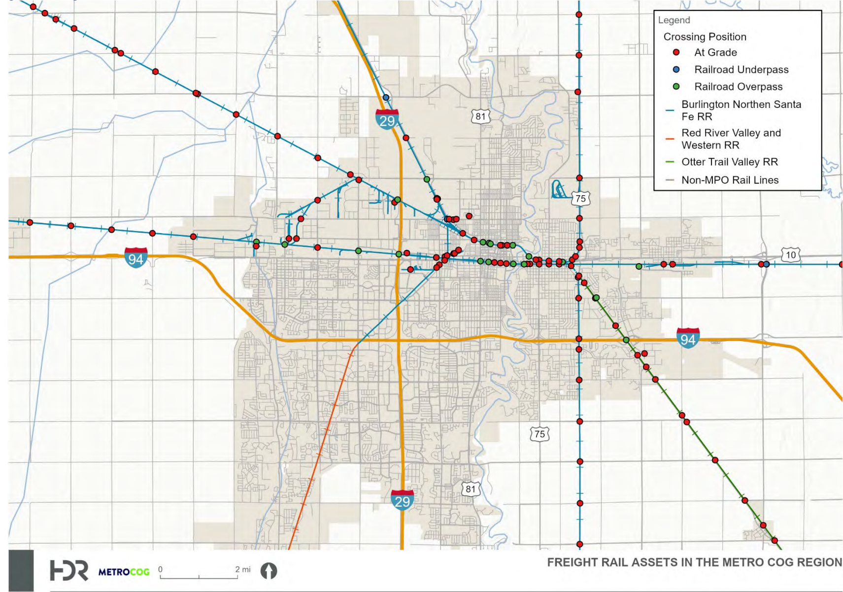
Figure 46: Freight Rail Assets in the MPA, Urban Inset
