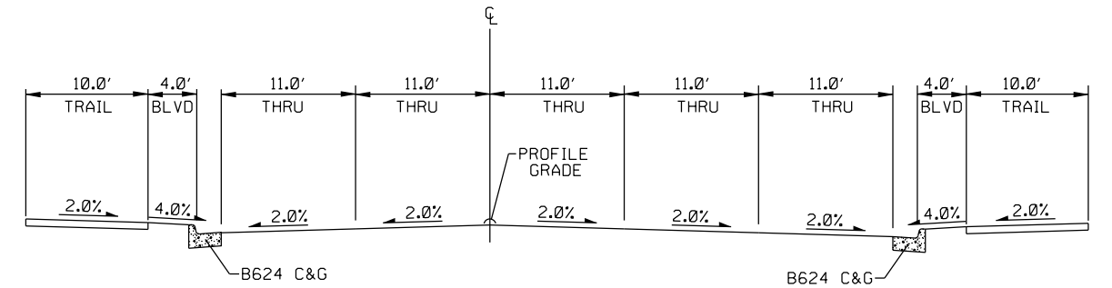
4-LANE URBAN RECONSTRUCTION WITH TRAIL
