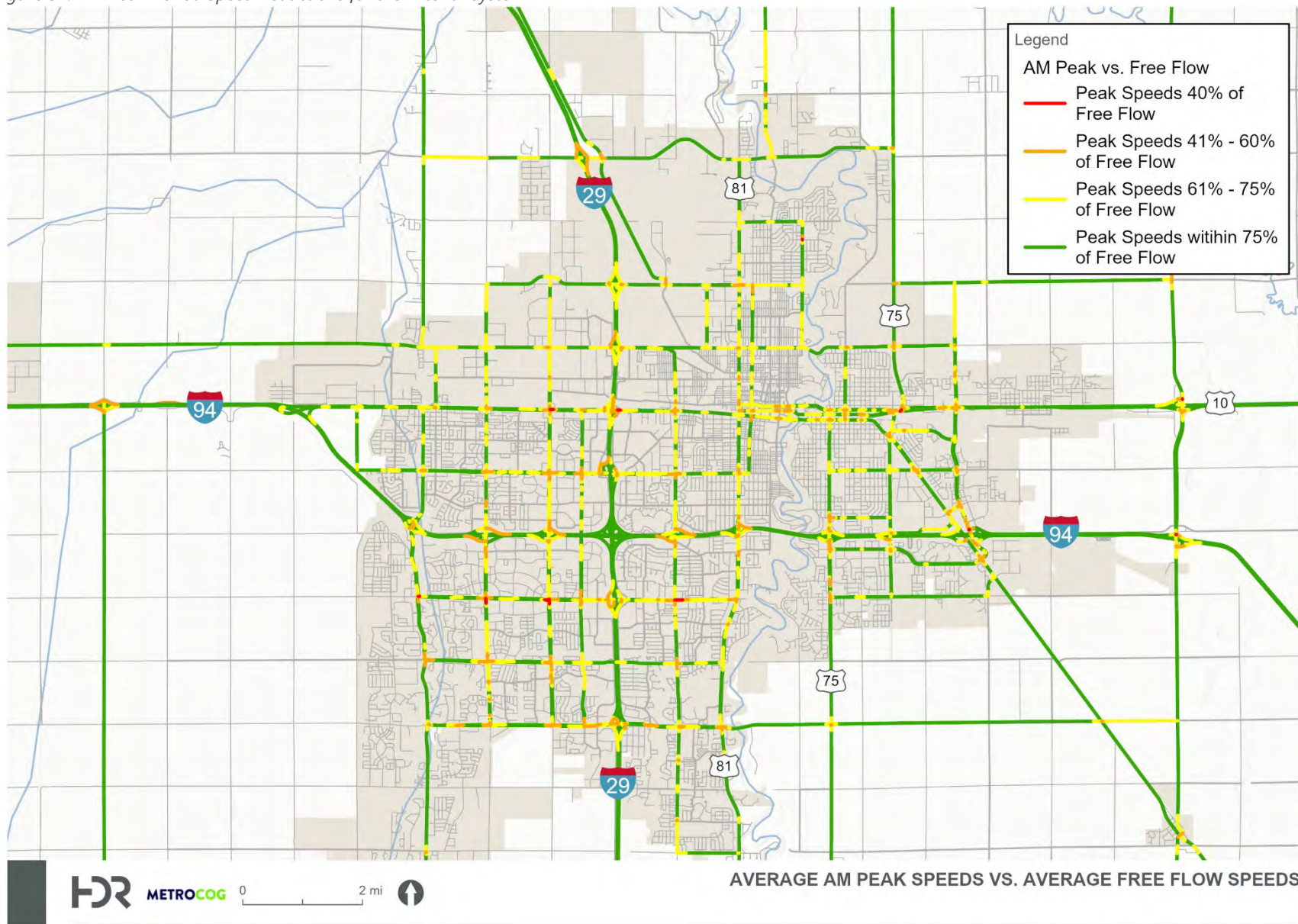
Figure 31: AM Peak Period Speed Reductions for the Arterial System
