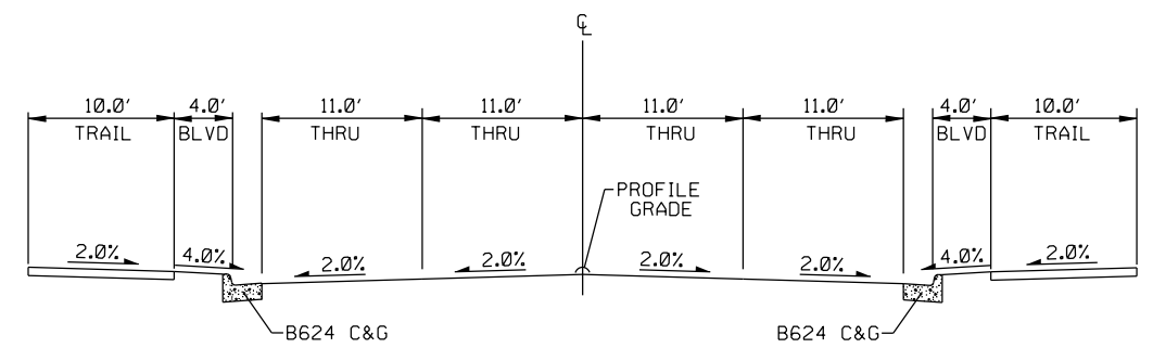
4-LANE URBAN RECONSTRUCTION WITH TRAIL
