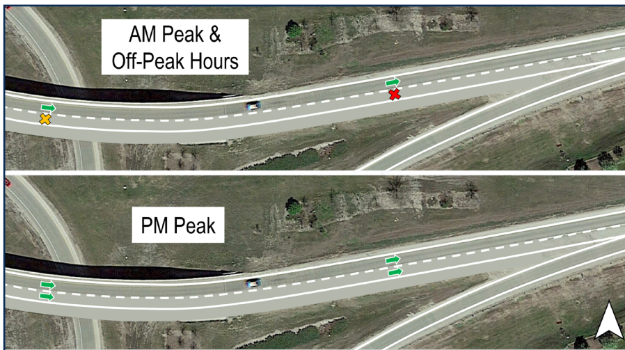
Figure 4.13. Dynamic Lane Assignment
