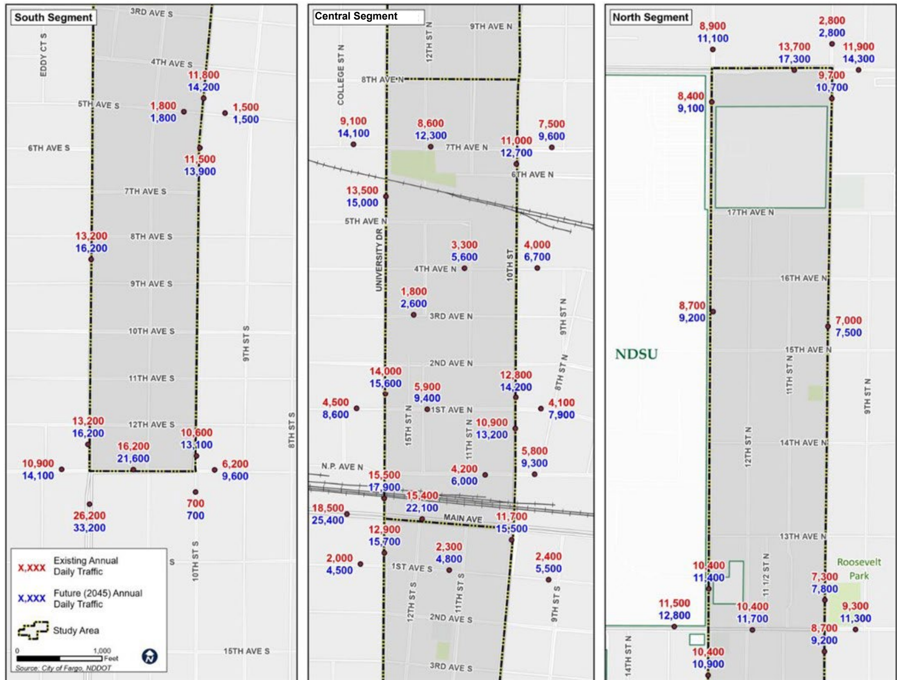
Figure 61: 2045 No Build Scenario Average Daily Traffic
